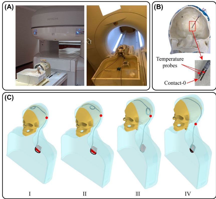
FIGURE 6 Phantom and experimental setup. A, Anthropomorphic phantom in the 1.2T vertical scanner (left) and a 1.5T horizontal scanner (right). B, DBS lead attached to temperature probes implanted into the skull. C, Schematic of phantom setup showing different trajectories (I, II, III, and IV) with different loop positions. The red dot represents the 40 cm mark measured from the intracranial end, representing the end-point for 40 cm wire
